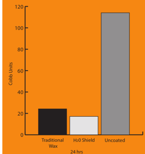
Cobb Test - Measure of Water Up-take
