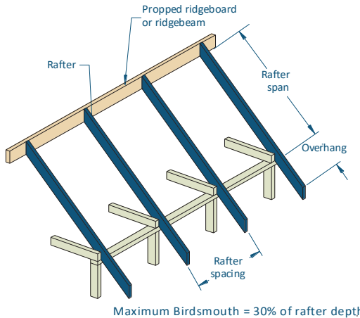
Maximum Birds-mouth = 30% of rafter depth
