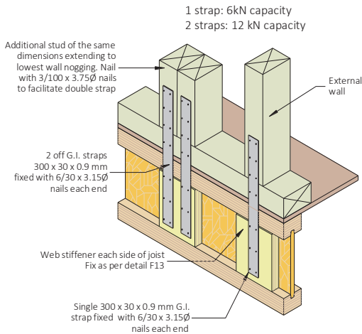
(b) SmartJoist parallel to upper bracing wall - via SmartRim and web stiffeners
