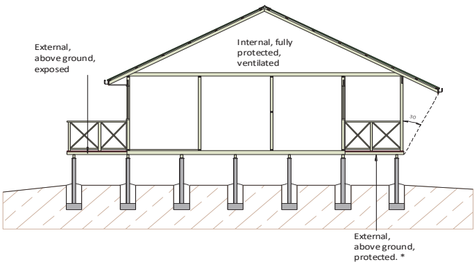
Definitions of exposure zones within a structure
