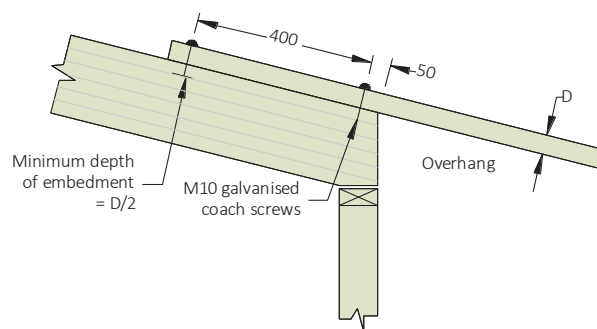
Figure 4 - Eaves over hang details for SmartLam GL17C
