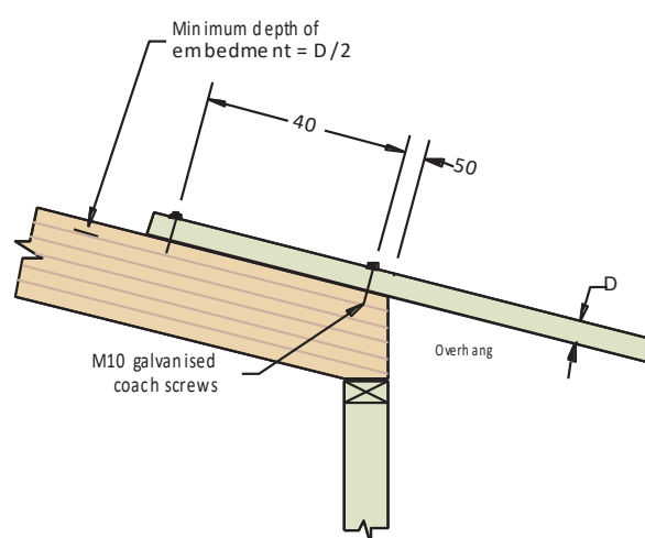
Figure 4 - Eaves overhang details for SmartLam GL18C
