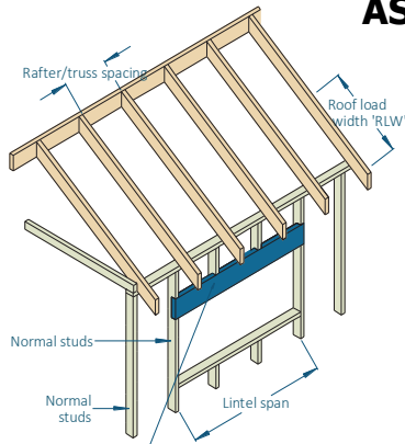
Single/Upper storey lintel
